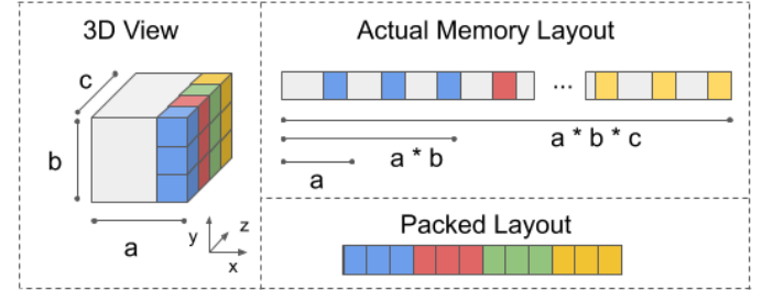
Fig. 6: Example of packing for a 3D region. In general, the linear storage order of the subdomain in memory causes the elements of the 3D region to be strided. The pack operation places only those elements in a dense buffer with some predetermined order.
